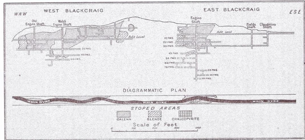
FIG. 7.—Sections showing the workings in the East and West Blackcraig Mines (Newton Stewart), with a diagrammatic plan showing the relations of the whin dyke to the ore.
